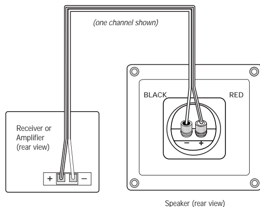
Figure 5. Wiring diagram shows polarity connections for one channel of a stereo or home theater system.
