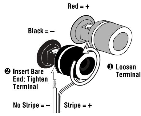
Figure 4. This example shows how to connect bare wires to the terminals.
